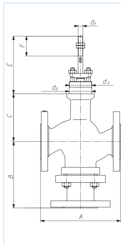
FIG.7. EXTERNAL AND CONNECTION DIMENSIONS
