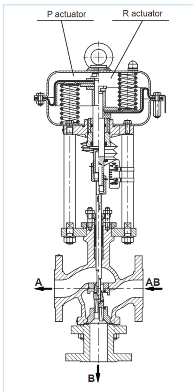
FIG.6. LP0-VA2013.R – DIVERTING
