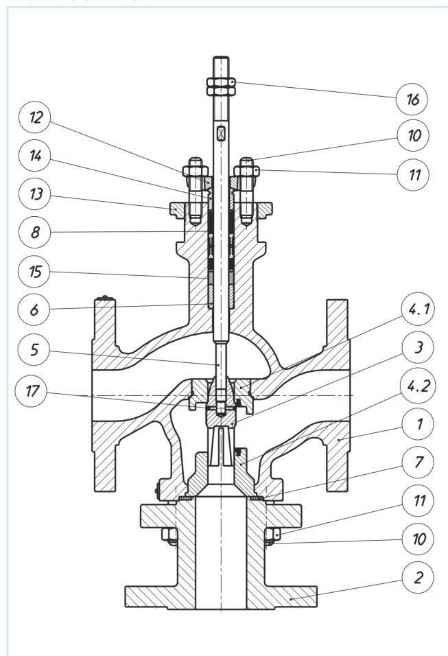
FIG. 1 - CONTROL VALVE
