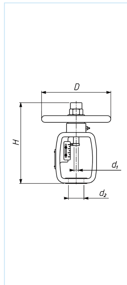
FIG. 9 HANDWHEEL TYPE 20
