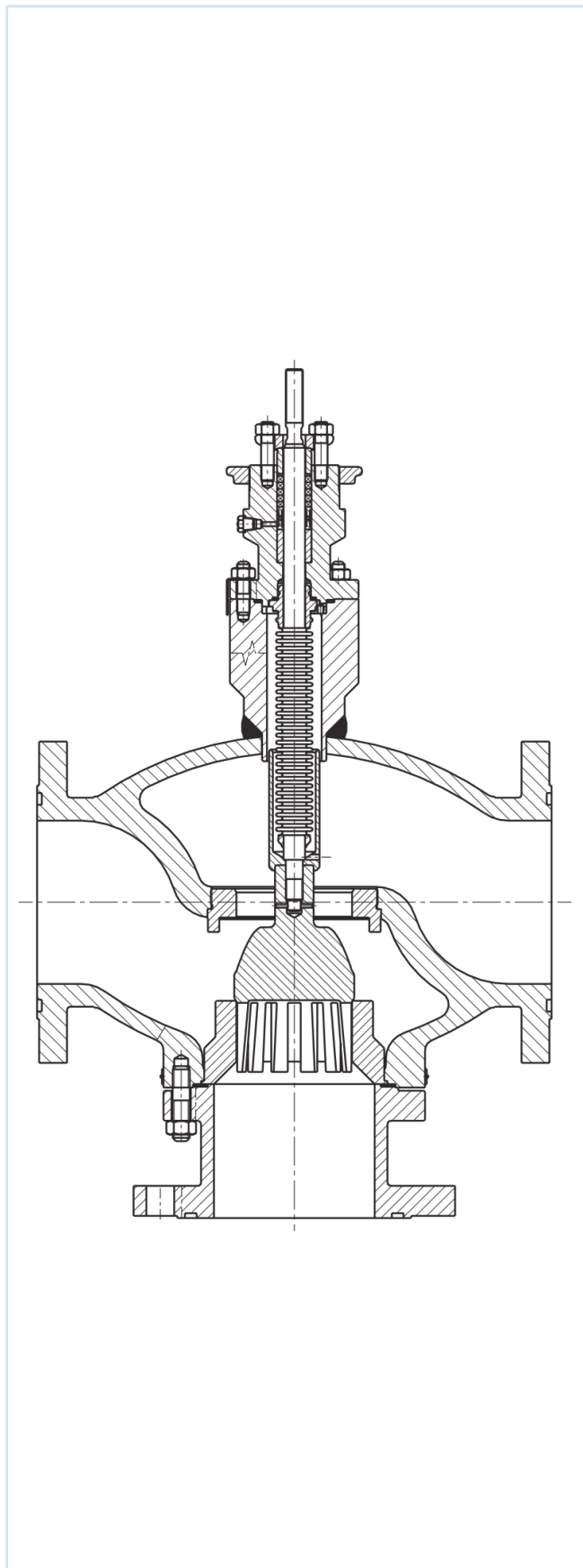
FIG. 3 - CONTROL VALVE WITH BELOW SEAL
