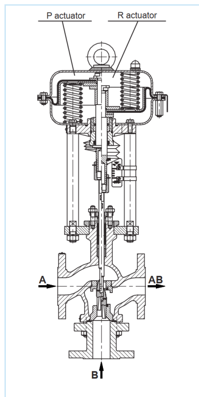
FIG. 5 LPO -VA2013.M - MIXING
