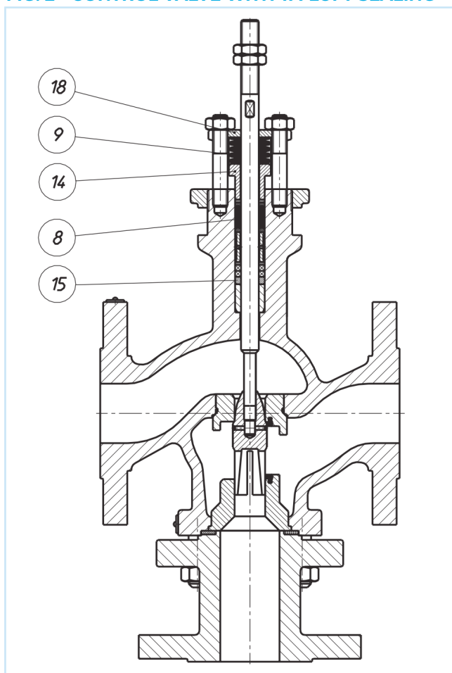
FIG. 2 - CONTROL VALVE WITH TA-LUFT SEALING
