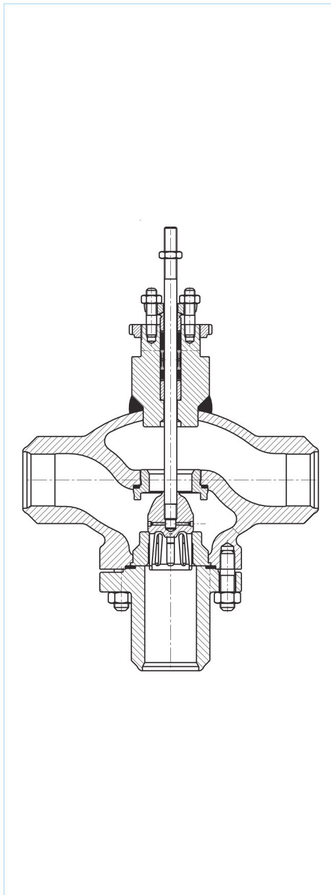
FIG. 4 - CONTROL VALVE WITH WELDED ENDS
